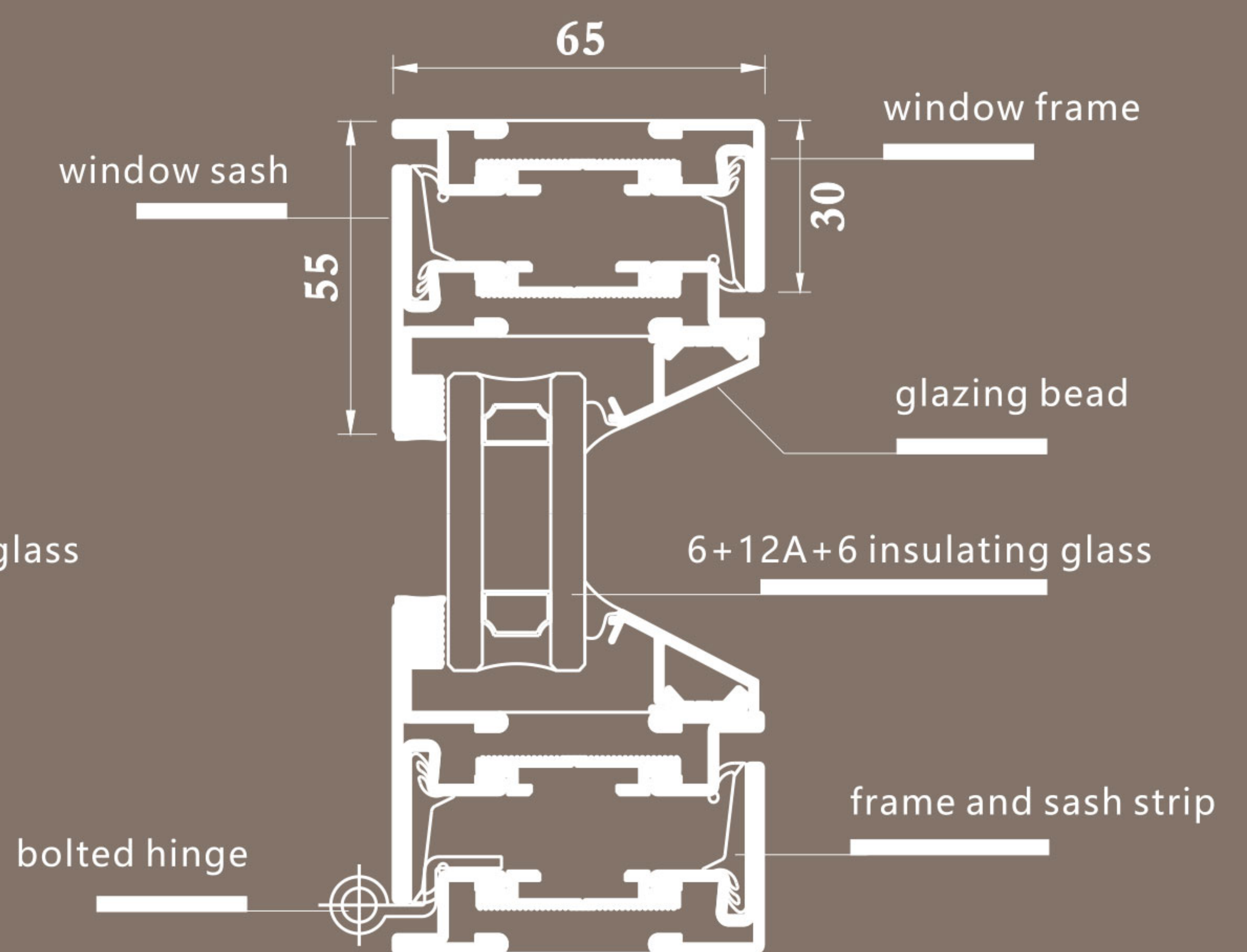
SLIM windows node
