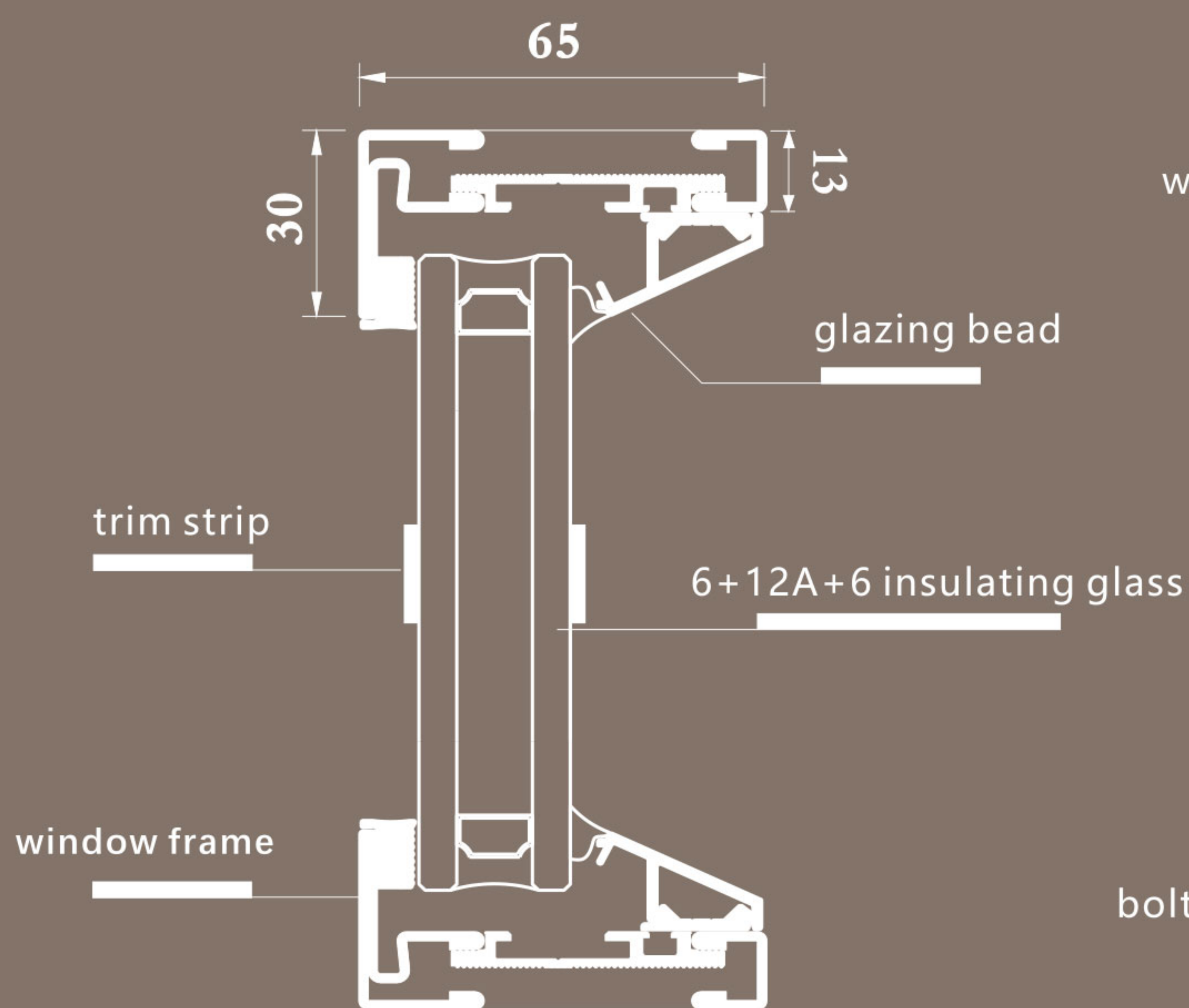
SLIM fixed windows node
